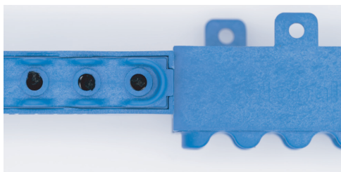
FIGURE 12A - Screw misaligned
