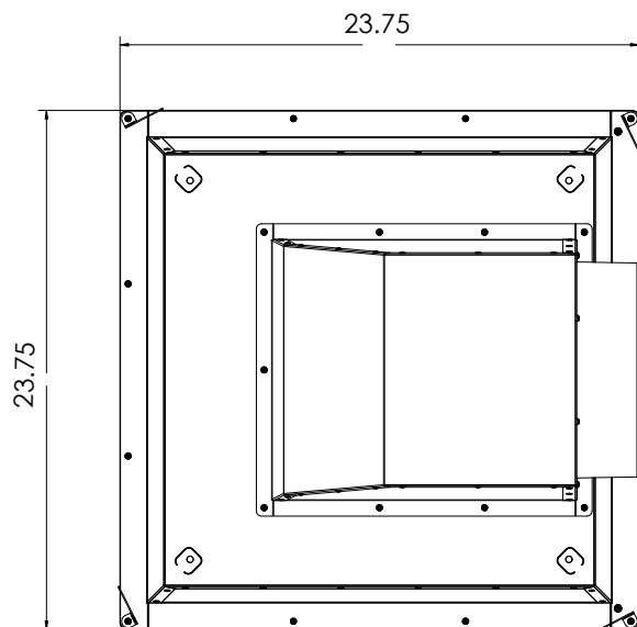
Plan View
